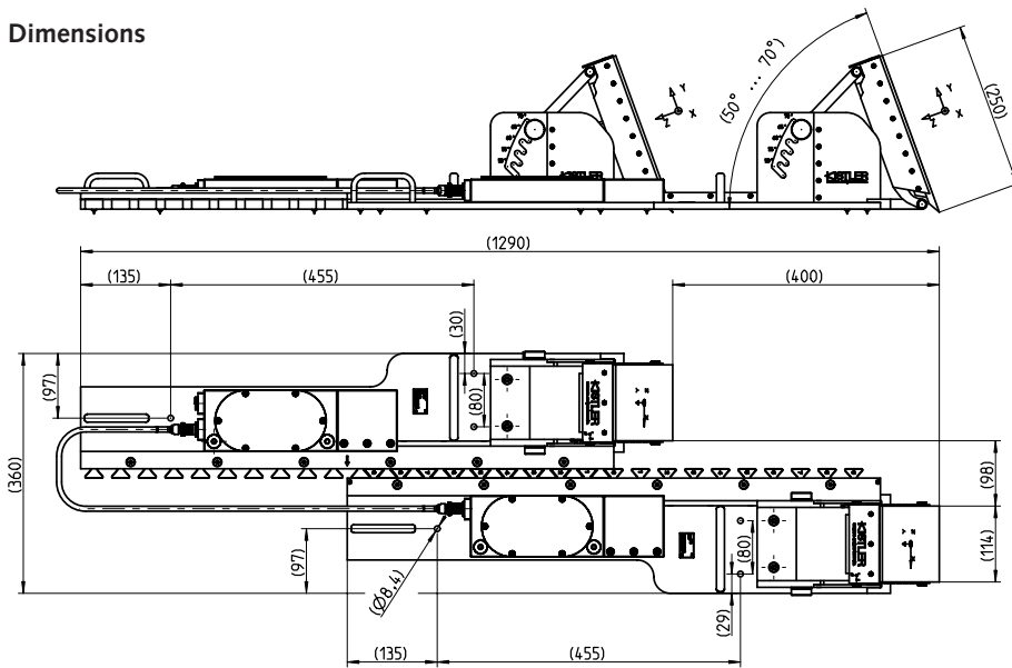
Fig. 1: Dimensions starting blocks Type Z20982
