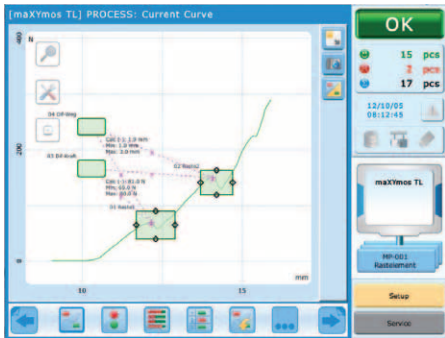
Application in product testing: Distance check between two breakover points of a fixing element. GETREF boxes provide the coordinates of the points to the CALCULATE objects. They in turn compute and evaluate the relevant distances in the force and displacement direction (current measurement curve).
