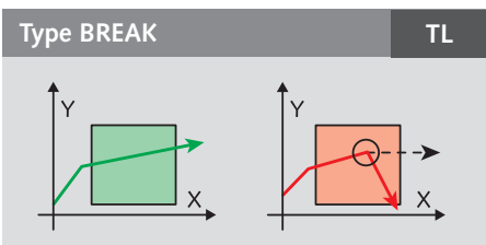
Provides NOK and online signal in case of sudden gradient change within an expectancy range (box), e.g. in case of tool breakage
