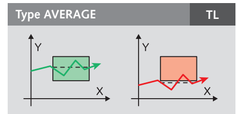
Evaluates the average of all Y-values in the box region
