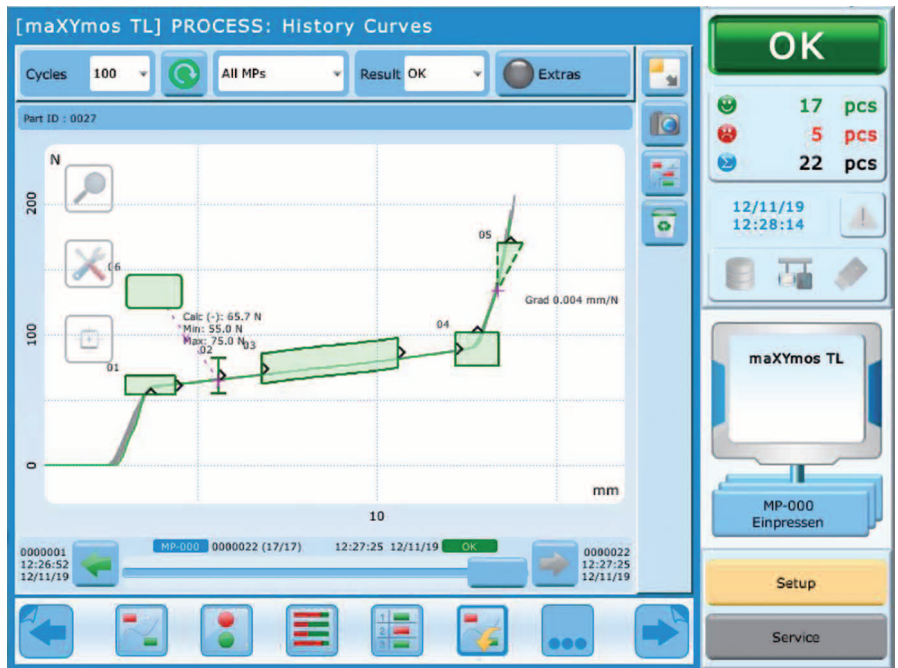
Screen TL: Curve history memory
