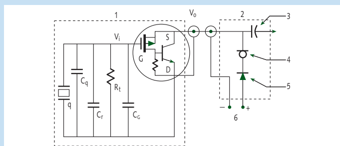
Fig. 5 Piezotron® circuit & coupler
