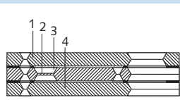
1 = top electrode 2 = spring 3 = mass 4 = bottom electrode
