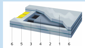
1 = top electrode 2 = frame 3 = spring 4 = mass 5 = bottom electrode 6 = glass layer
