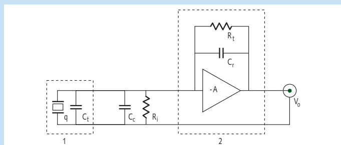
Fig. 4 Simplified charge amplifier model
