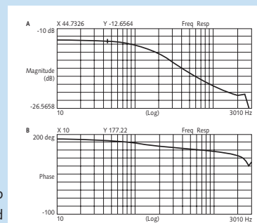
Fig. 4b Tuned system
